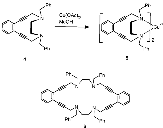
Scheme 4. 1,2-Benzodiyne with amino coordination sites
