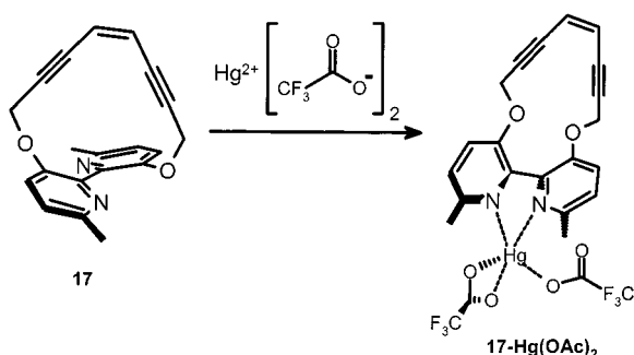
Scheme 6. Activation of enediyne 17 by formation of a mercury complex
