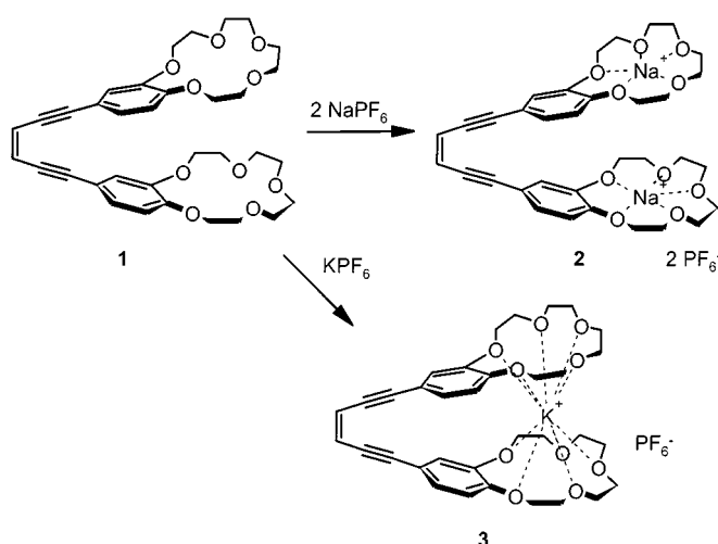
Scheme 3. Enediyne bis-crown ethers and their sodium and potassium complexes
