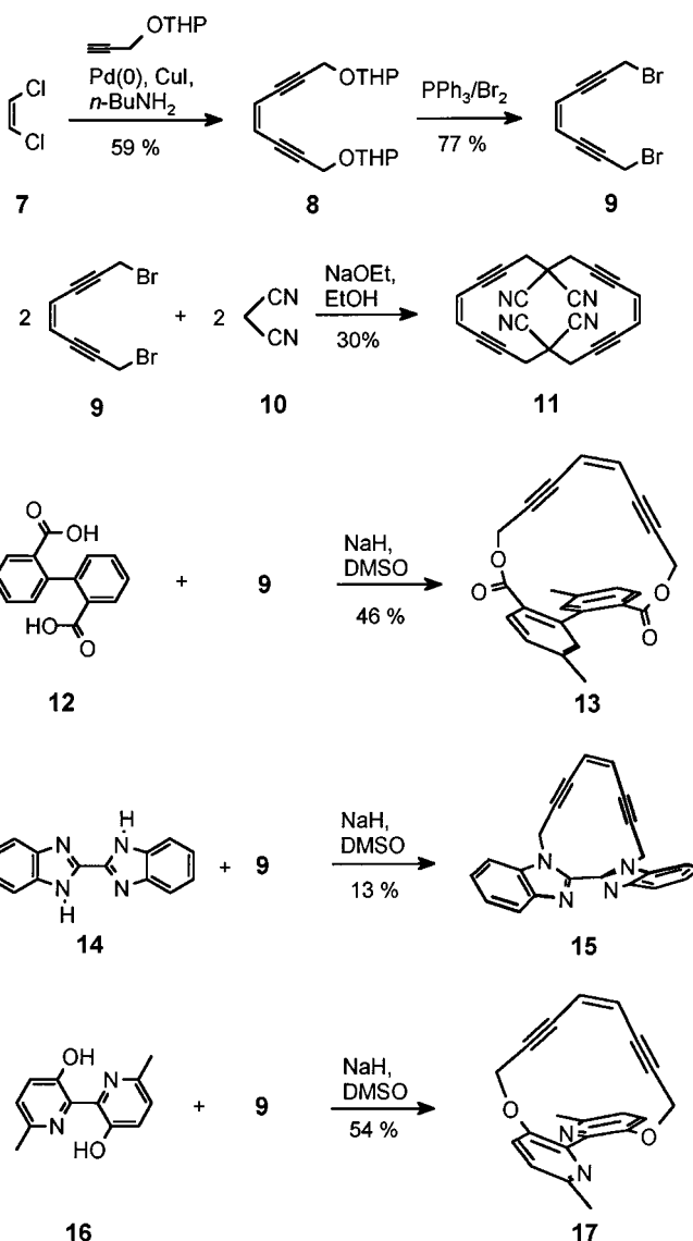
Scheme 5. Synthesis of macrocyclic enediynes by substitution reaction
